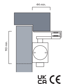
Fig.66 Parallel arm push side mount
