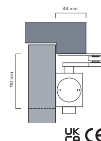
Fig.66 Parallel arm push side mount
