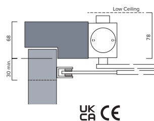
Fig.61 Transom mount push side
