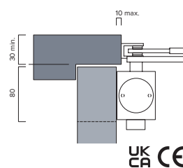
Fig.1 Door mount pull side
