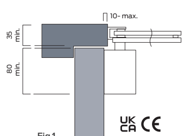
Fig.1 Door mount pull side
