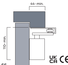
Fig.66 Parallel arm push side mount
