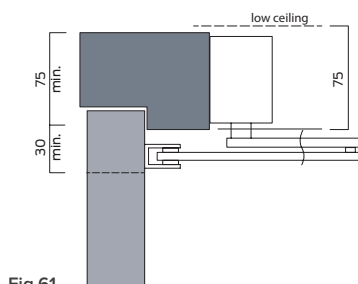
Fig.61 Transom mount push side
