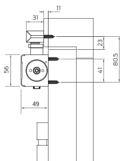
Door mount - Pull side (trimplate version)
