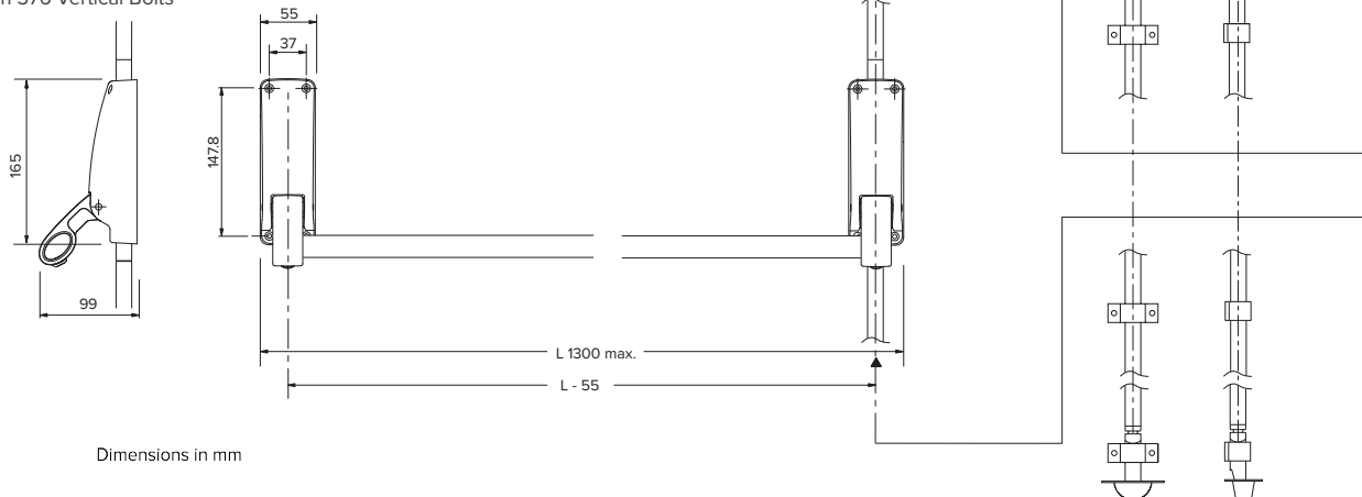
Briton 376 Vertical Bolts
